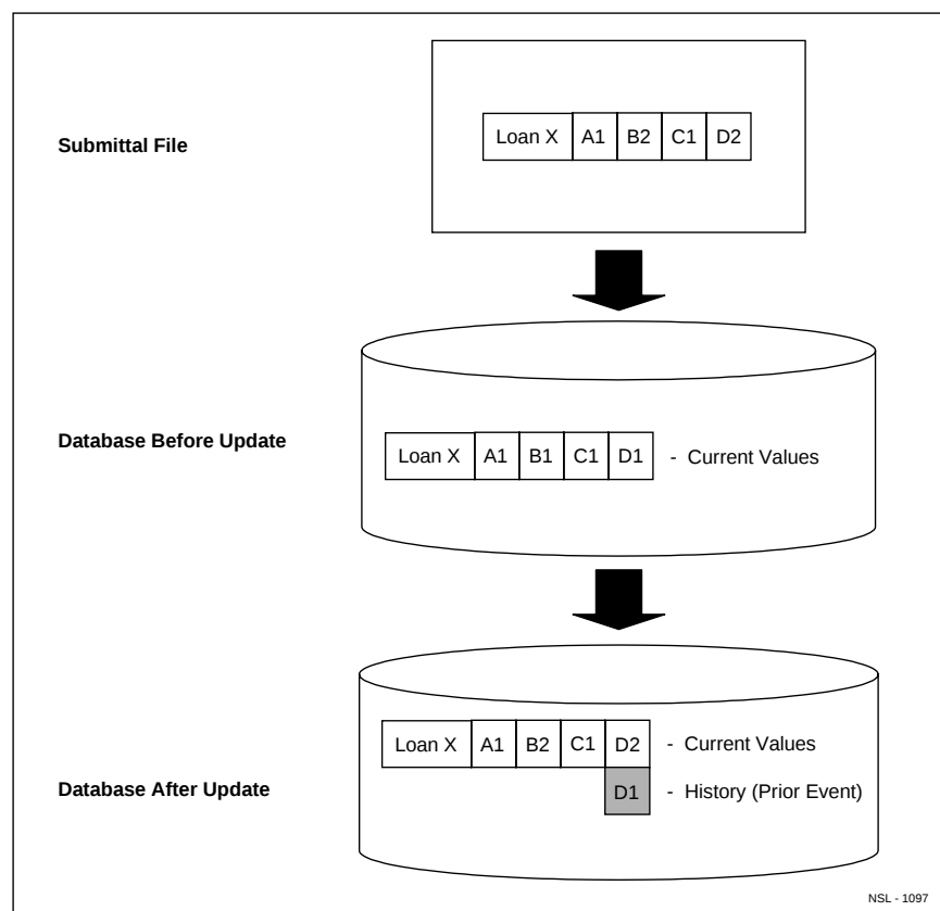
Figure 6–3, NSLDS Update (1 of 2)
