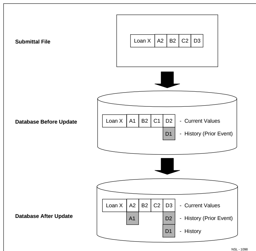
Figure 6–4, NSLDS Update (2 of 2)
