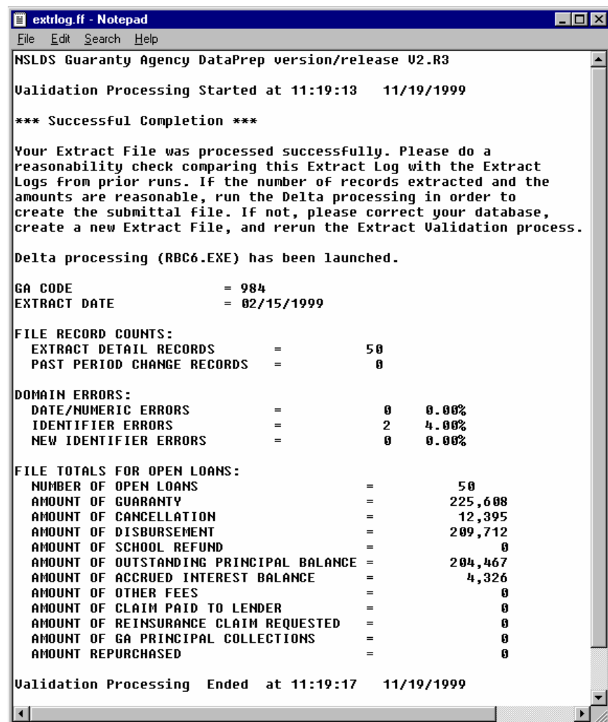
Figure 10-3, Extract Validation Log Report
