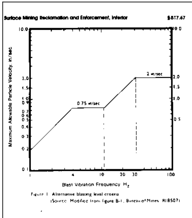
Figure 1. Alternative blasting level criteria. (Source: Modified from figure B-1, Bureau of Mines R18507)
