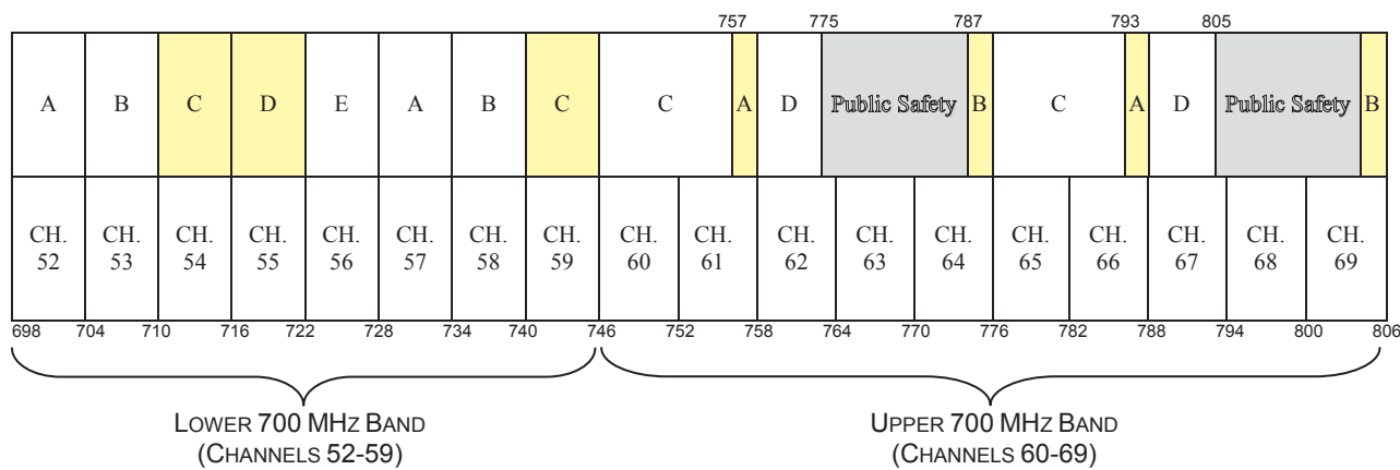
FIGURE 1: REVISED 700 MHz BAND PLAN FOR COMMERCIAL SERVICES
