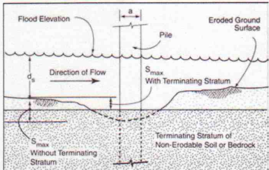
Figure 10 Local Scour
