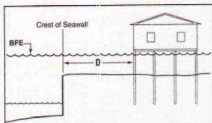
Figure 4a Erosion Control Device, D < 30 Feet
