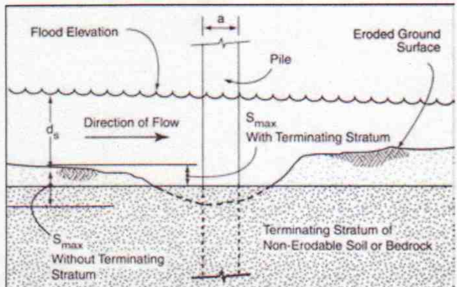
Figure 10 Local Scour
