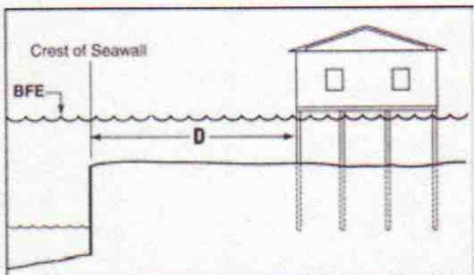
Figure 4b Erosion Control Device, D ≥ 30 Feet
