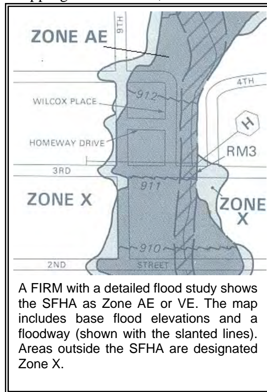
Figure 410-1. FIRM terminology.
