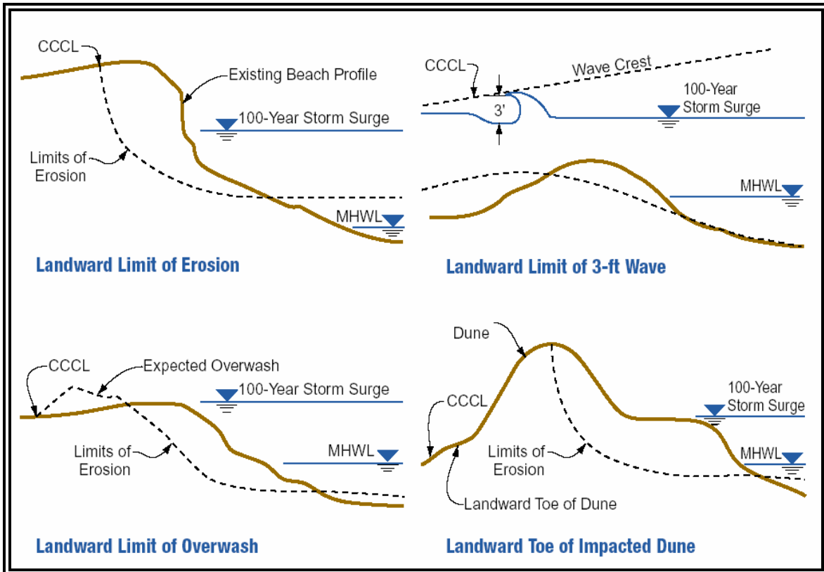
Criteria for locating the Coastal Construction Control Line (from Federal Emergency Management Agency, 2000a, p. G-12).
