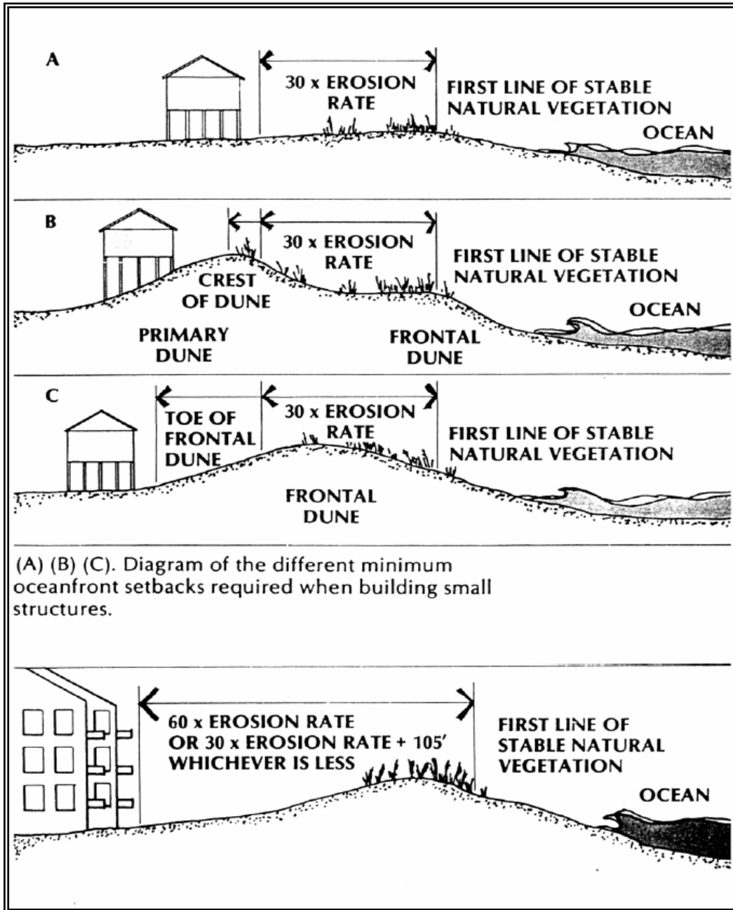
Illustration of North Carolina's setback regulations (from Federal Emergency Management Agency, 2000a, p. G-14).
