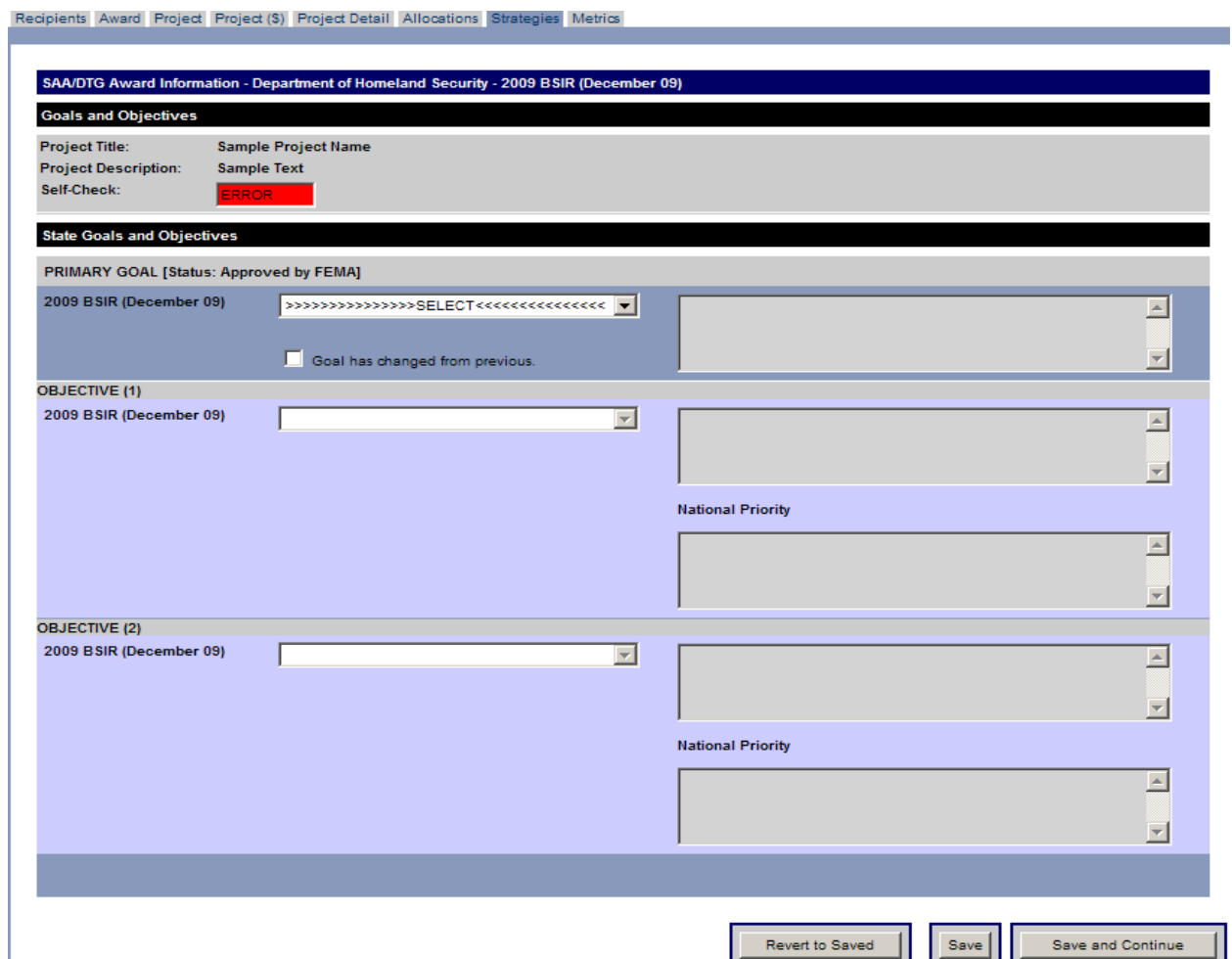
Figure 68: Strategies Tab
