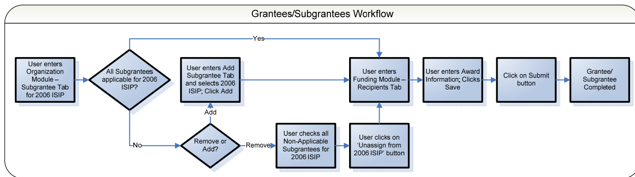
Figure 32: Grantees/Subgrantees Workflow
