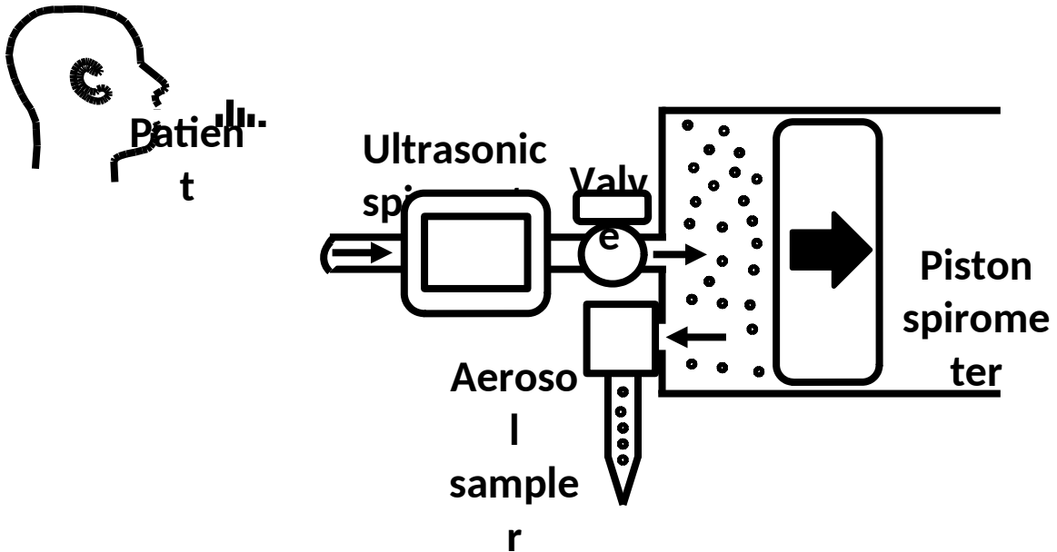
Cough aerosol particle collection system
