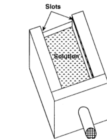
Figure 3 — Slot Hood for Dip Tank
