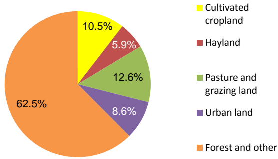
Figure 2. Distribution of land use/cover types in the Chesapeake Bay watershed
