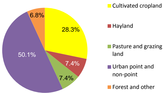
Figure 5. Percentage of average annual phosphorus loads delivered to rivers and streams in the Chesapeake Bay watershed, by source
