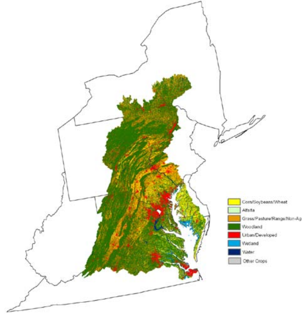
Figure 1. Location of the Chesapeake Bay watershed
