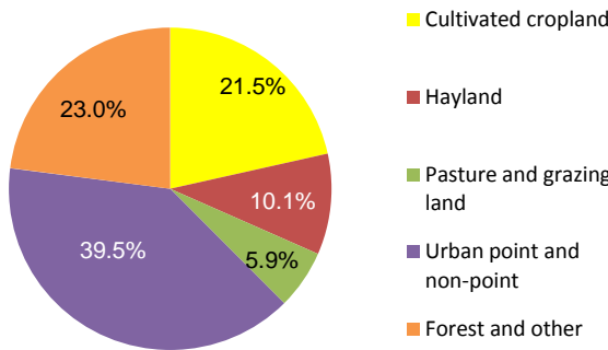
Figure 3. Percentage of average annual sediment loads delivered to rivers and streams in the Chesapeake Bay watershed, by source
