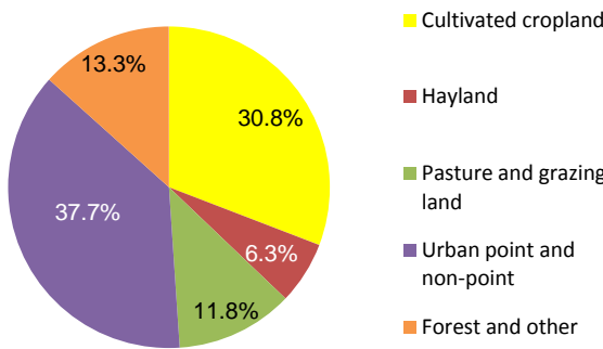
Figure 4. Percentage of average annual nitrogen loads delivered to rivers and streams in the Chesapeake Bay watershed, by source
