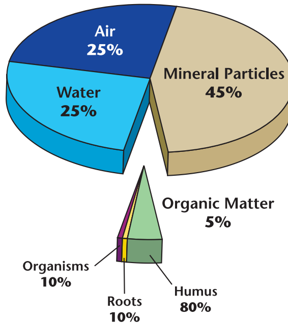
Figure A-1. Average composition of soil.
