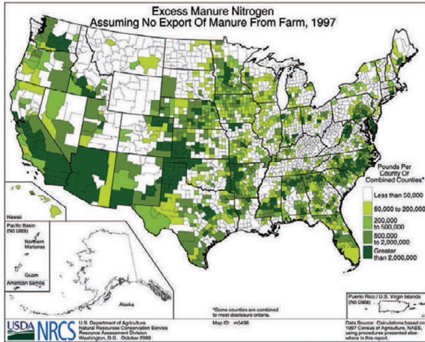
Figure 6-4. Excess manure nitrogen.
