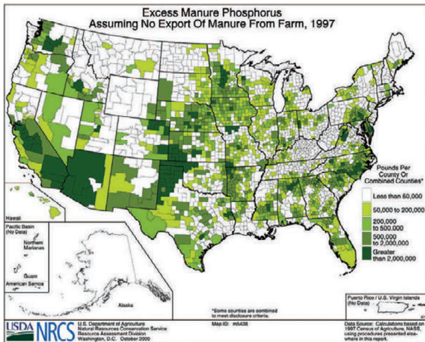
Figure 6-5. Excess manure phosphorus.
