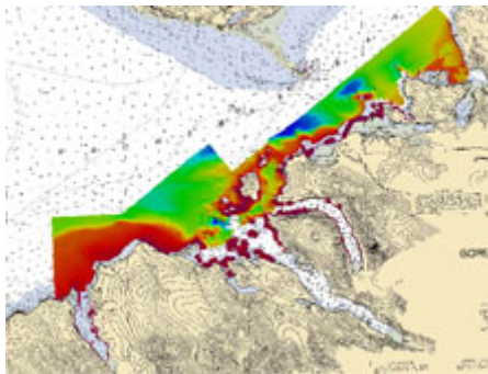
Figure 11 - Bathymetric Map of Kachemak Bay, AK
