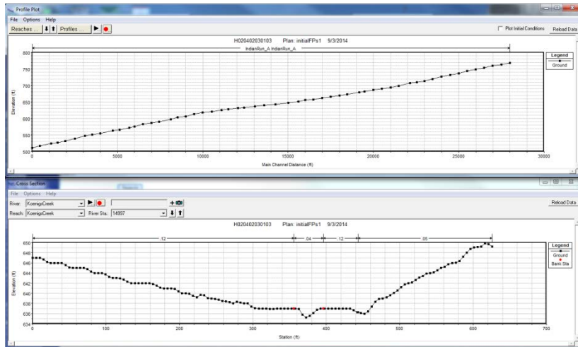
Figure 15 - Stream Profile (top) and Cross Section Profile (bottom)
