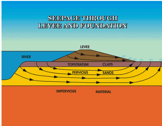
Figure 16 - Seepage Around a Levee
