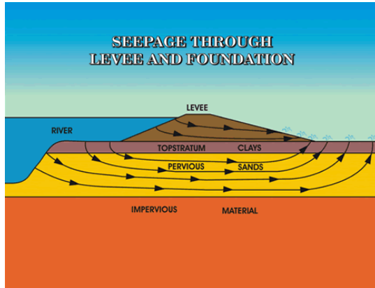
Figure 16 - Seepage Around a Levee
