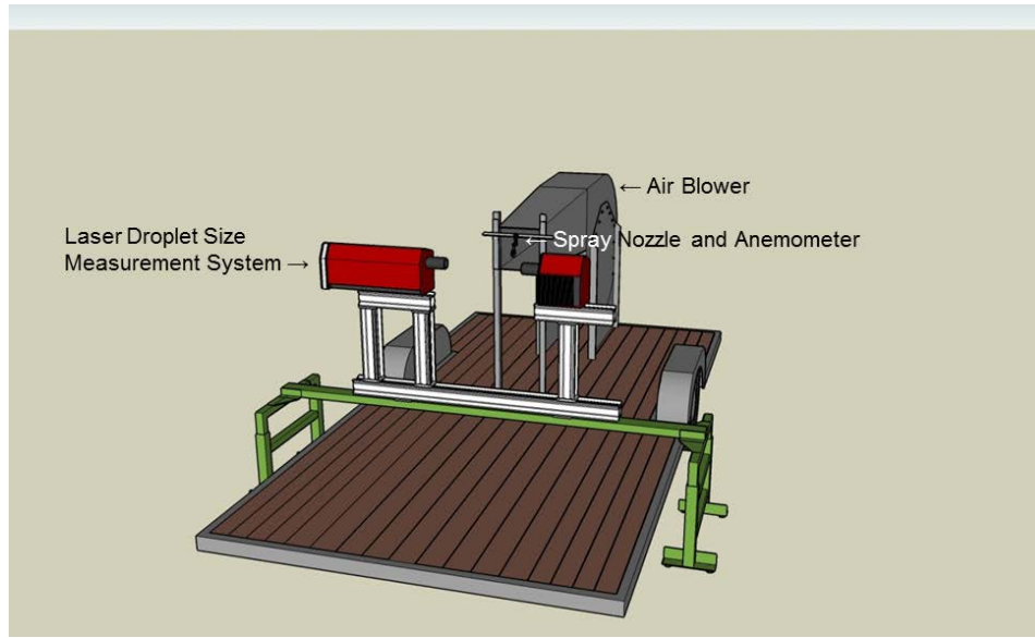
Figure 1. Example of typical inside view of instrumentation setup for wind tunnel at a low or high speed wind tunnel.
