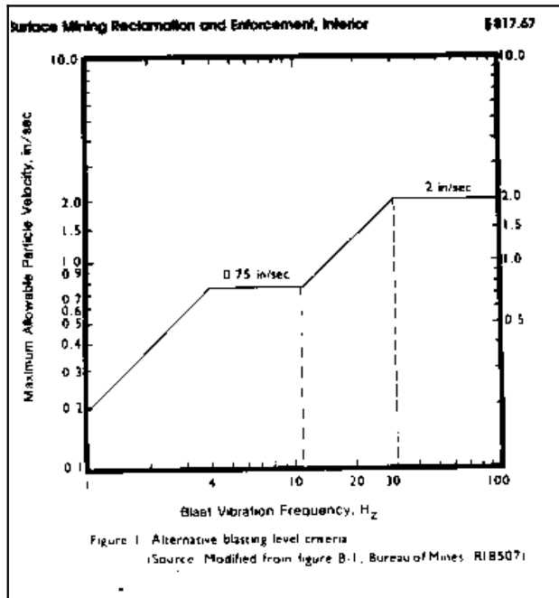
Figure 1. Alternative blasting level criteria (Source: Modified from figure B-1, Bureau of Mines R18507)
