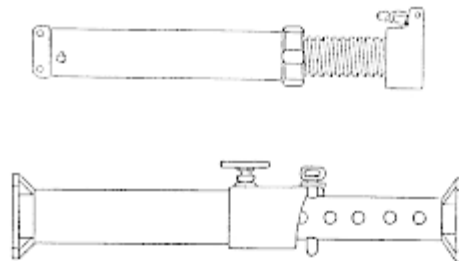
Figure 2. Pneumatic/hydraulic Shoring
