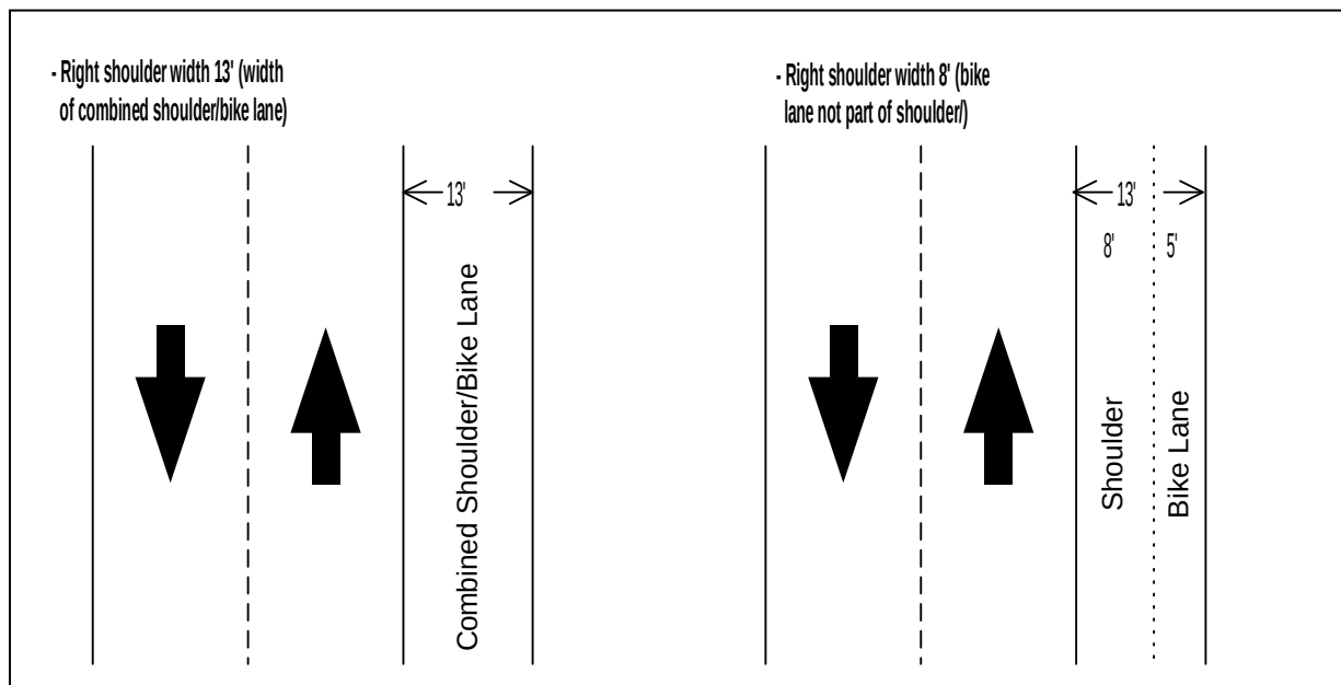
Figure IV-6C. Shoulder Type/Width
