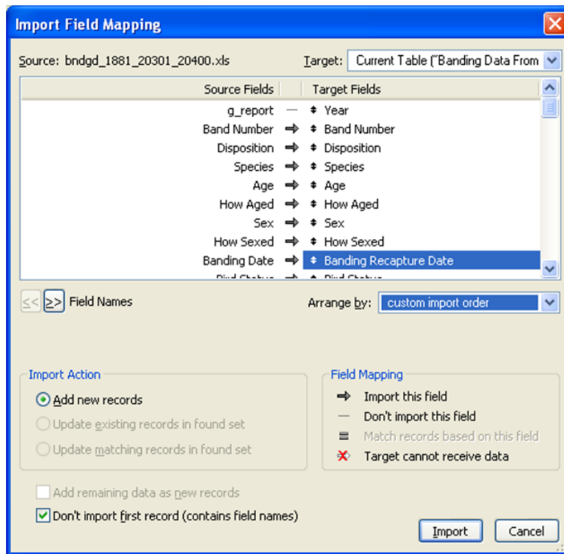
Figure 12.2. Import Field Mapping Screen
