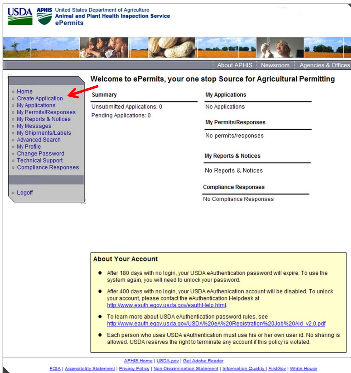
Figure 2: Home Page
