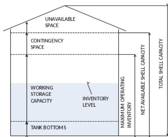
Figure 2. Schematic of Cavern Storage Capacity and Stocks
