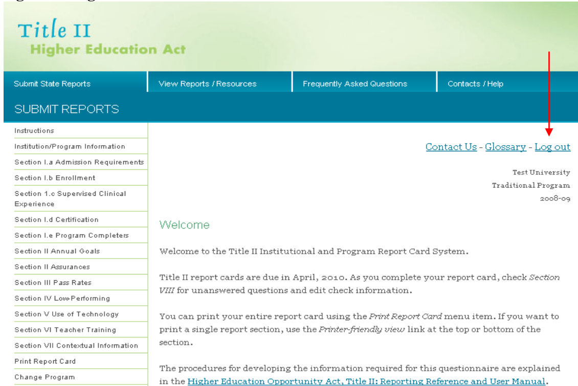
Figure 6. Log out
