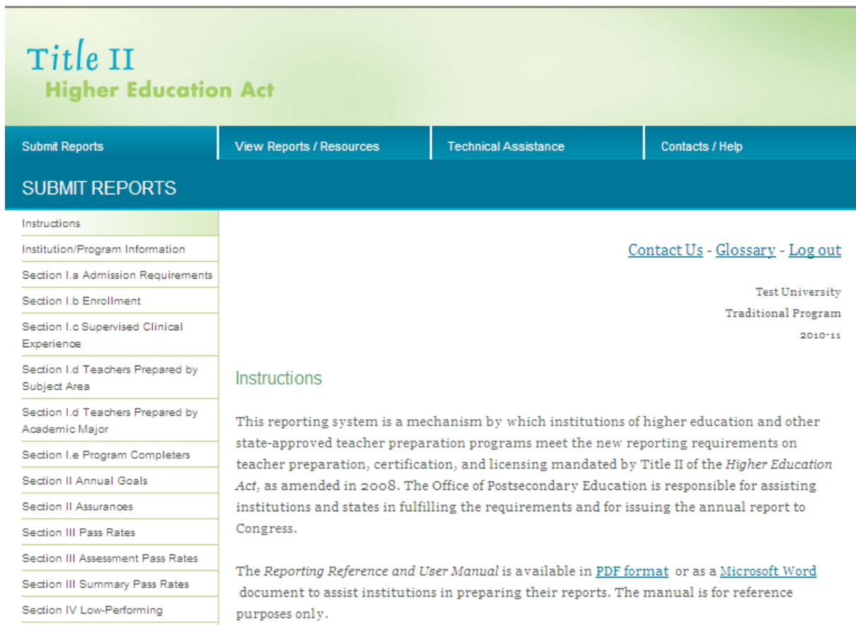
Figure 12. Main menu
