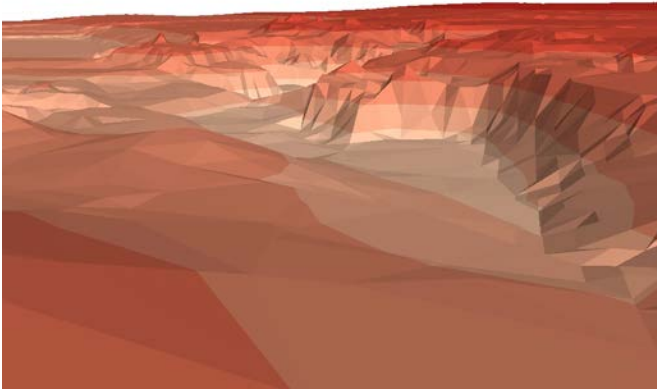
Figure 1. Topographic bedrock map (five times vertical exaggeration) in the vicinity of the recharge ponds based on the additional geophysical investigation
