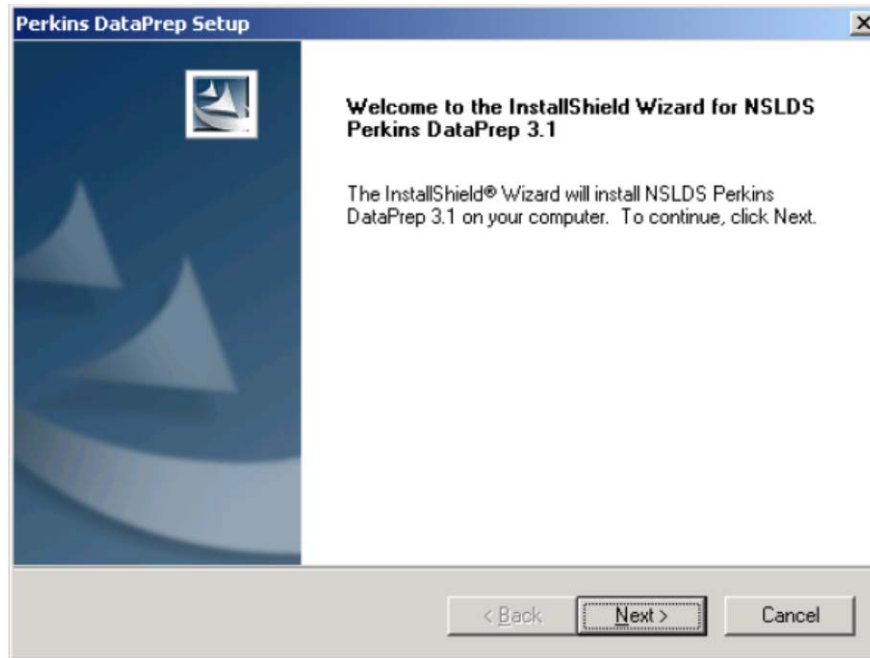
Figure 5-3: InstallShield Wizard
