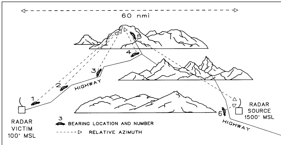
FIGURE 14-2. RADAR INTERFERENCE DF EXAMPLE
