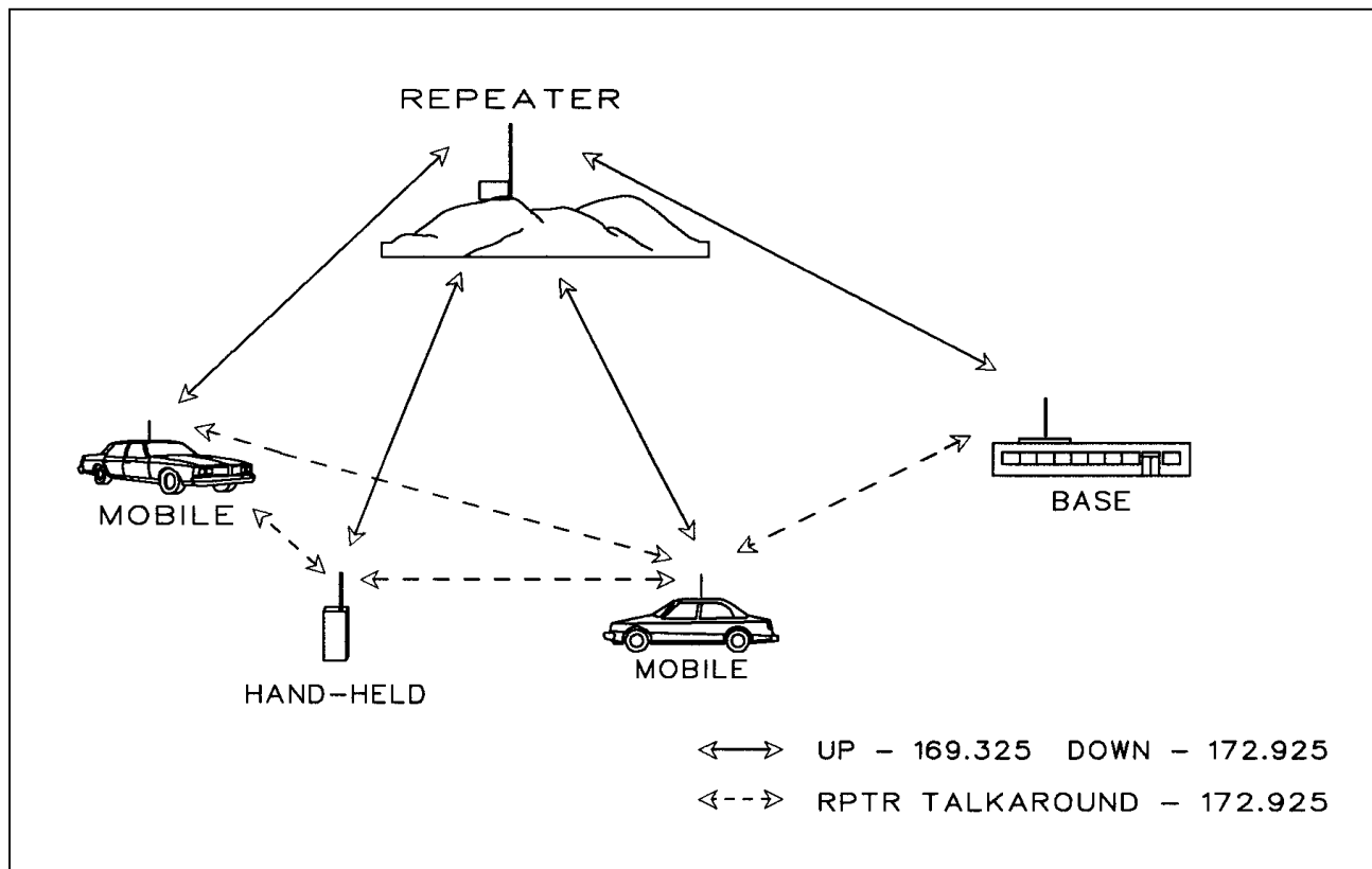
FIGURE 17-2. EXAMPLE OF A REPEATER/BASE/PORTABLE/MOBILE FM SYSTEM
