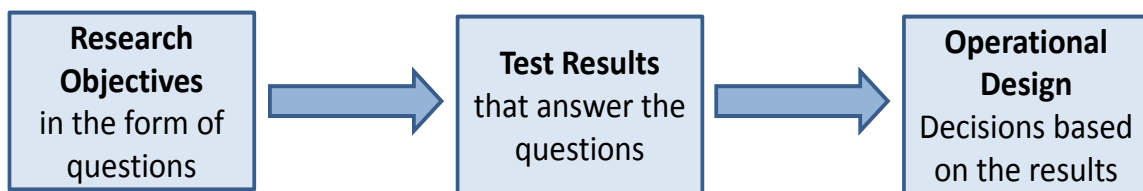
FIGURE 1: RESEARCH PROCESS
