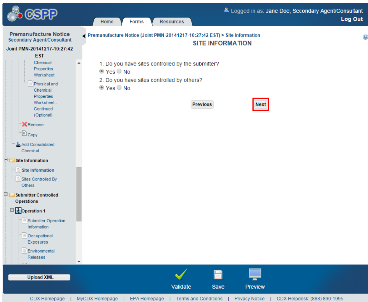
Exhibit 4-25: Submitter Controlled Site Information Screen (Joint PMN)
