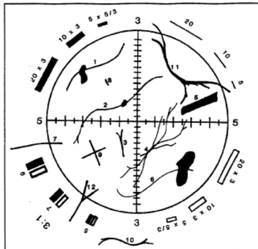
Figure 1: Walton-Beckett Graticule with some explanatory fibers.
