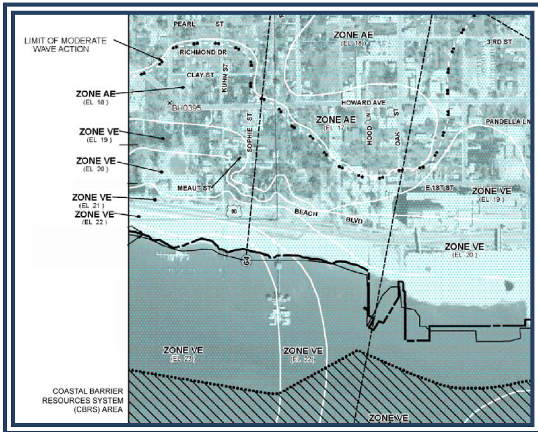
Figure 410-2. An example of a coastal FIRM.
