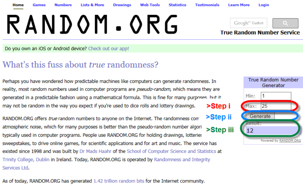
Figure 1: Illustration of www.Random.Org web site. The portions of the random number generator used in steps i-iii of (question 10b) are circled.
