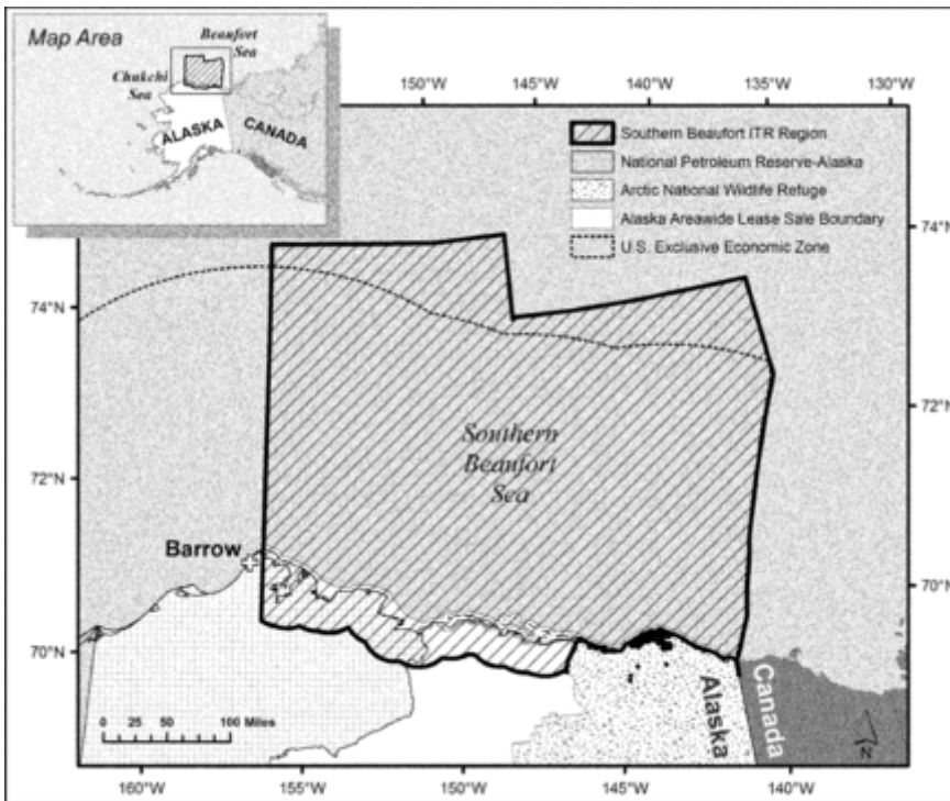
Figure 1. Map of the Beaufort Sea ITR region.
