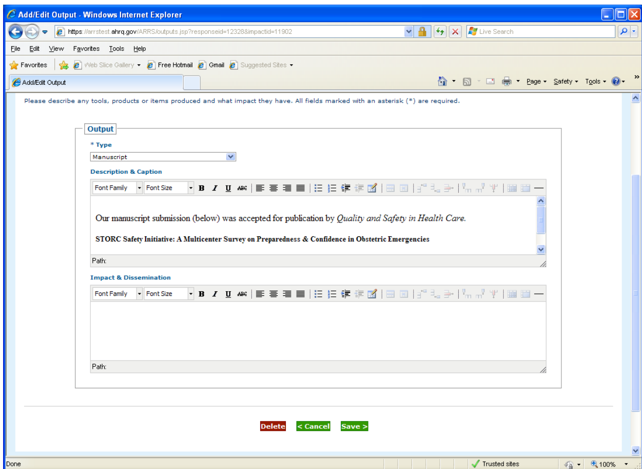
Figure 19: Output Page
