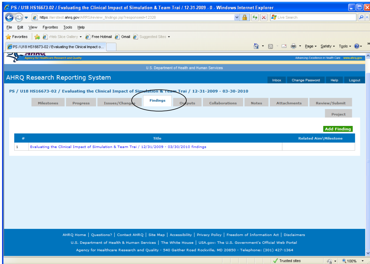
Figure 16: Findings Tab
