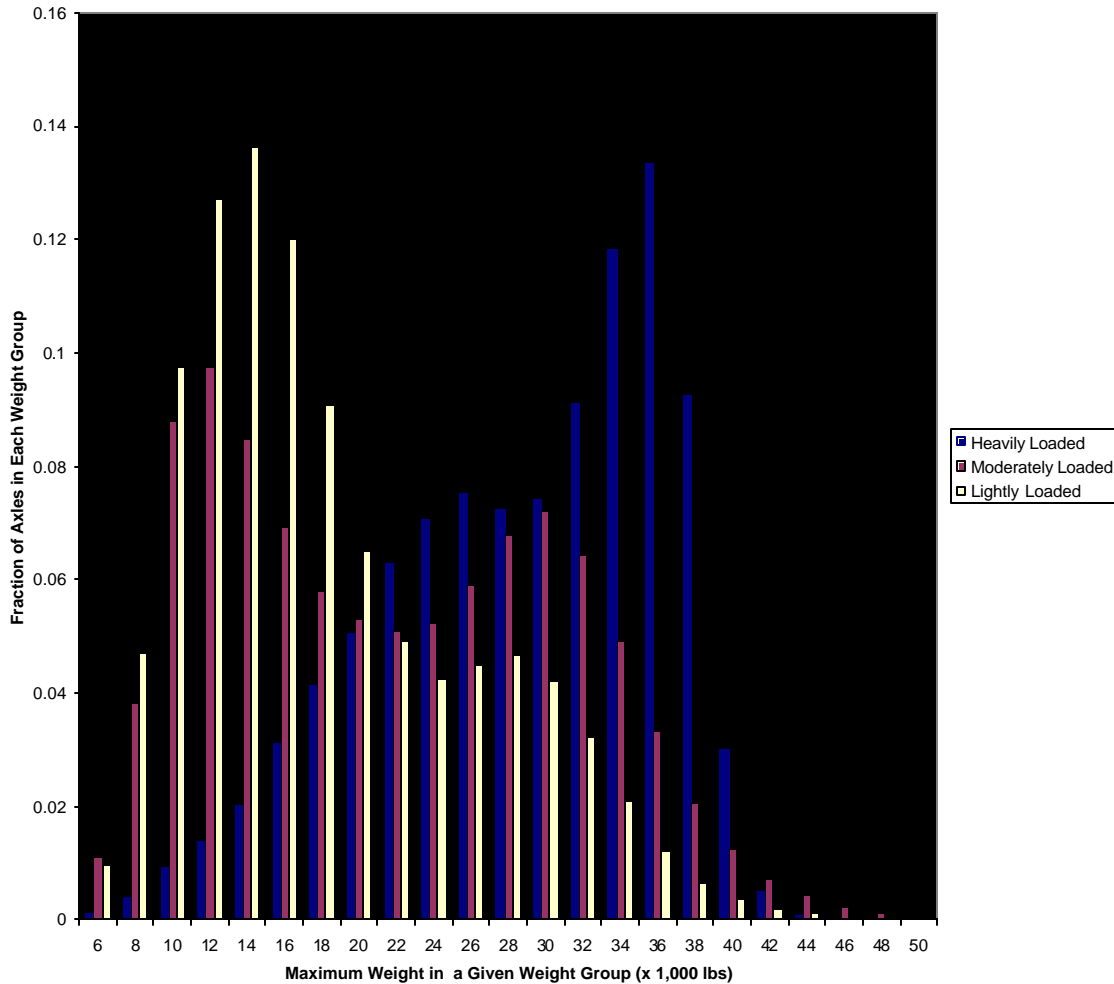
Figure 5-3-1: Tandem Axle Load Distributions At Three Sites With Different Loading Conditions. The Case For Truck Weight Road Groups
