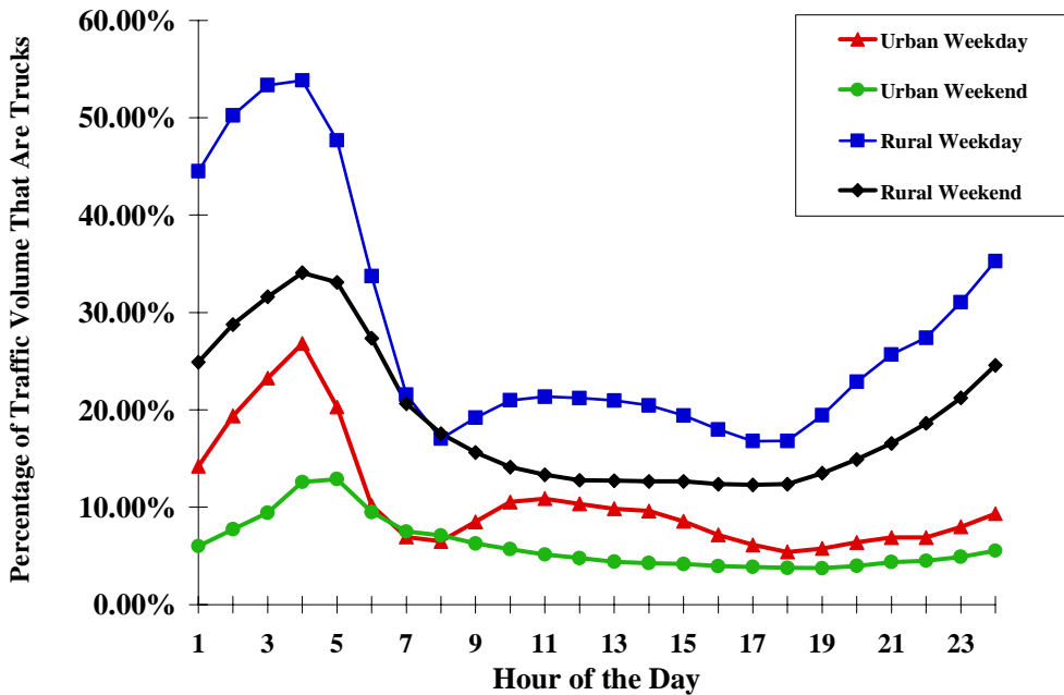
Figure 2-2-2 Weekday/Weekend Truck Percentages
