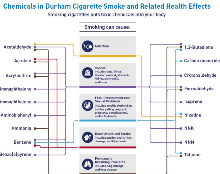
Figure F-2. Chemicals in Smoke
