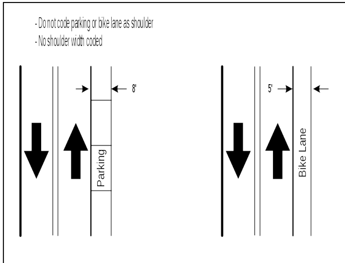
Figure IV-6A. Shoulder Type/Width
