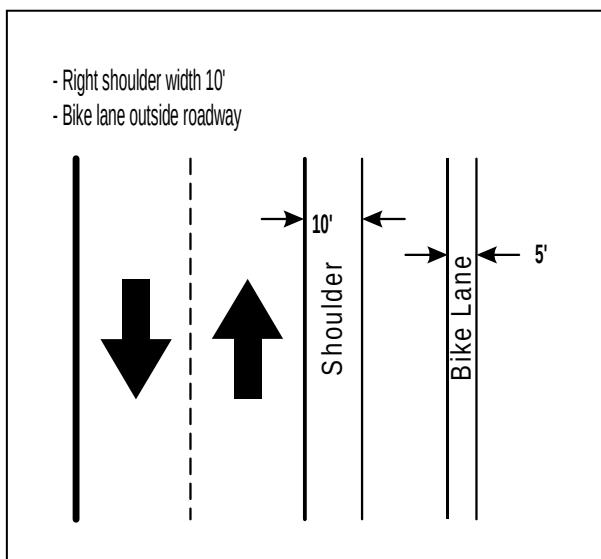
Figure IV-6B. Shoulder Type/Width
