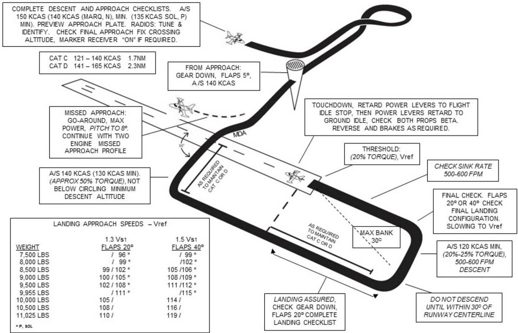
Figure A-27 MU-2B MARQUISE (-60), SOLITAIRE (-40), N (-36A), P (-26A) CIRCLING APPROACH AT WEATHER MINIMUMS
