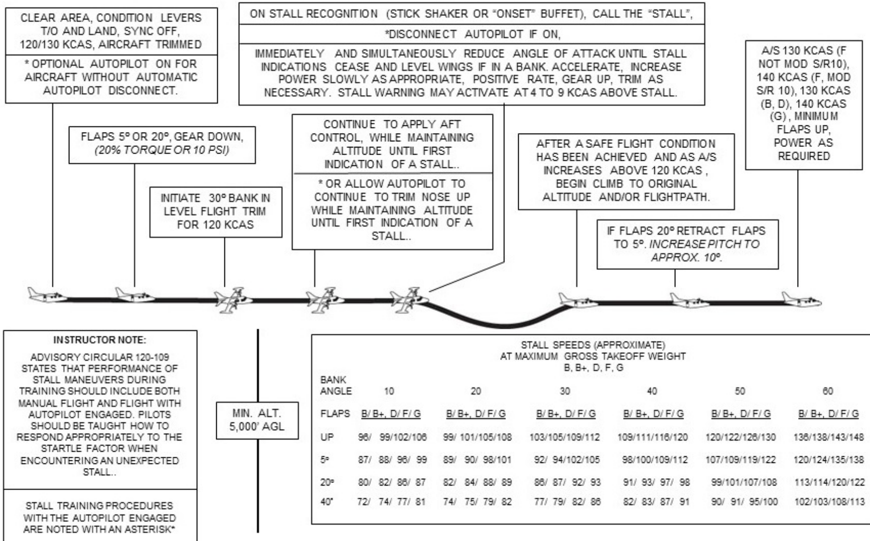
Figure C-9 MU-2B B, D (-10), F (-20), G (-30) APPROACH TO STALL TAKEOFF CONFIGURATION 15-30° BANK
