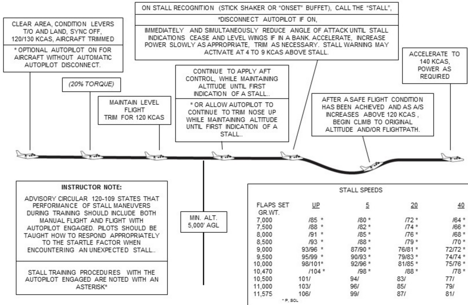
Figure A-8 MU-2B MARQUISE (-60), SOLITAIRE (-40), N (-36A), P (-26A) APPROACH TO STALL CLEAN CONFIGURATION / WINGS LEVEL
