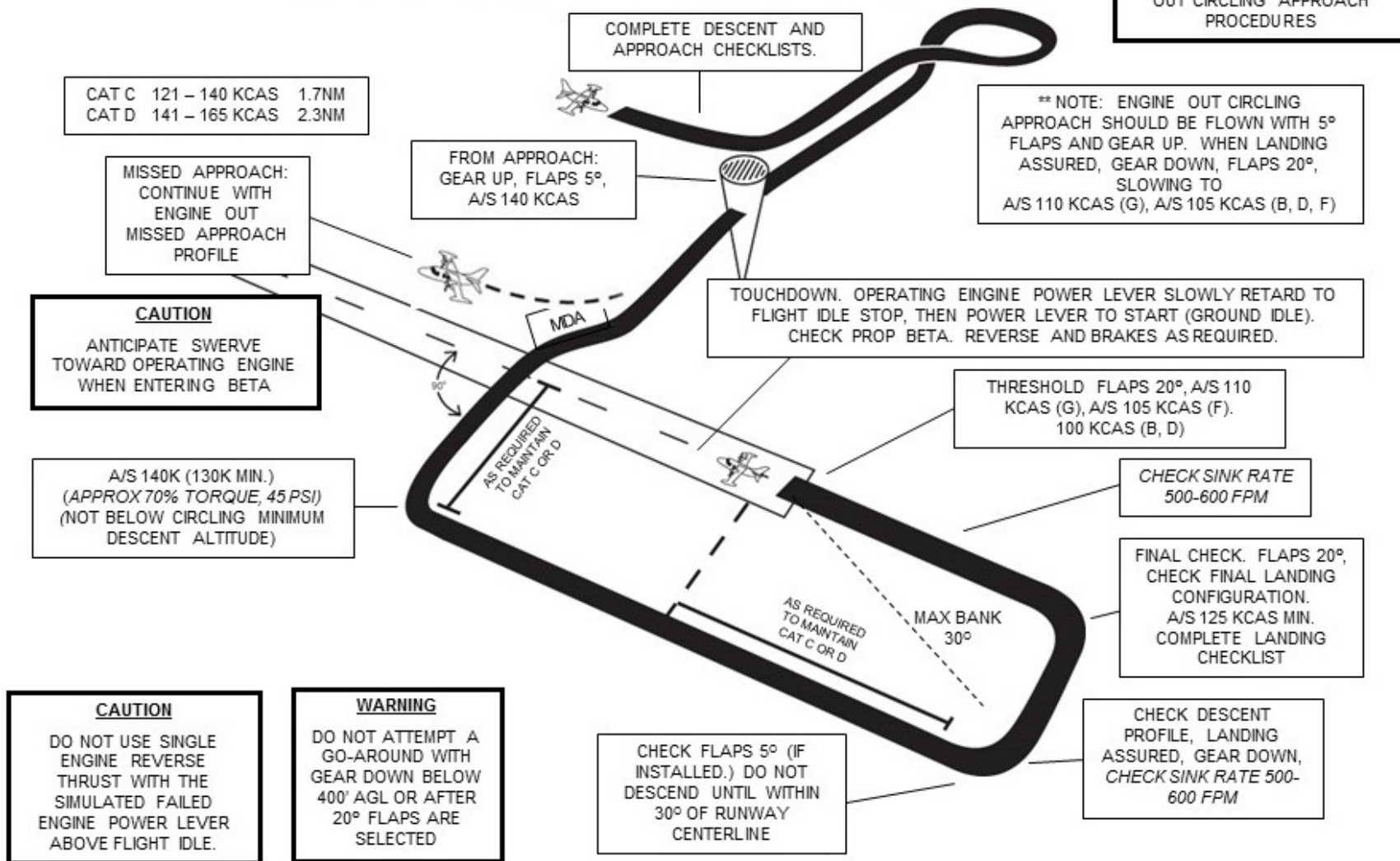
Figure C-28 MU-2B B, D (-10), F (-20), G (-30) ONE ENGINE INOPERATIVE CIRCLING APPROACH AT WEATHER MINIMUMS
