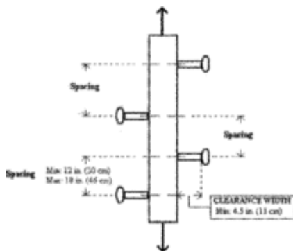
Figure D-6 – Step Bolt Spacing
