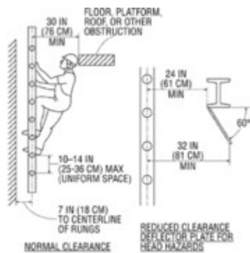
Figure D-5 -- Fixed Ladder Clearances
