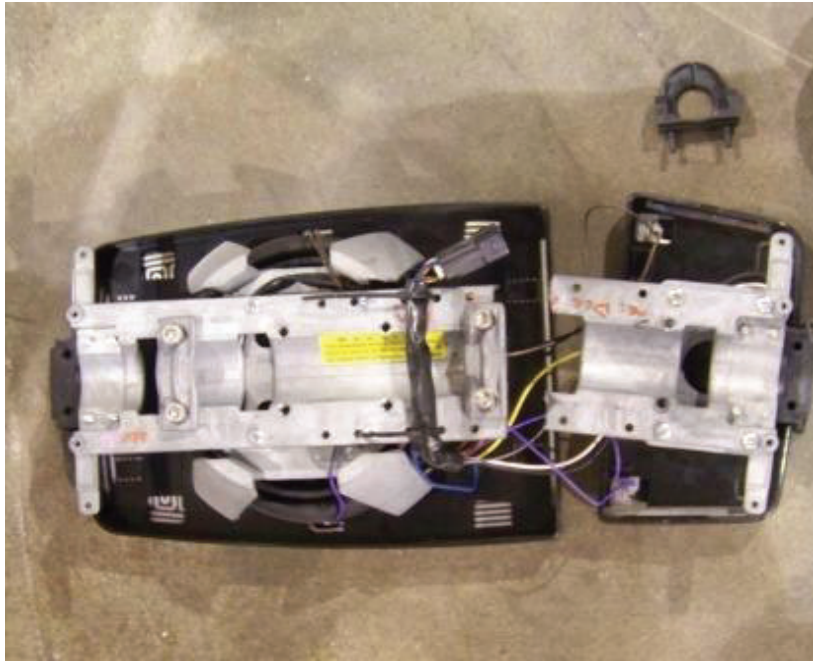
BROKEN REAR VIEW MIRROR MOUNTING BLOCK (4,815 TEST MILES)
