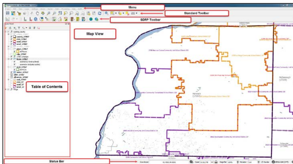
Figure 35. GUPS Main Page Layout
