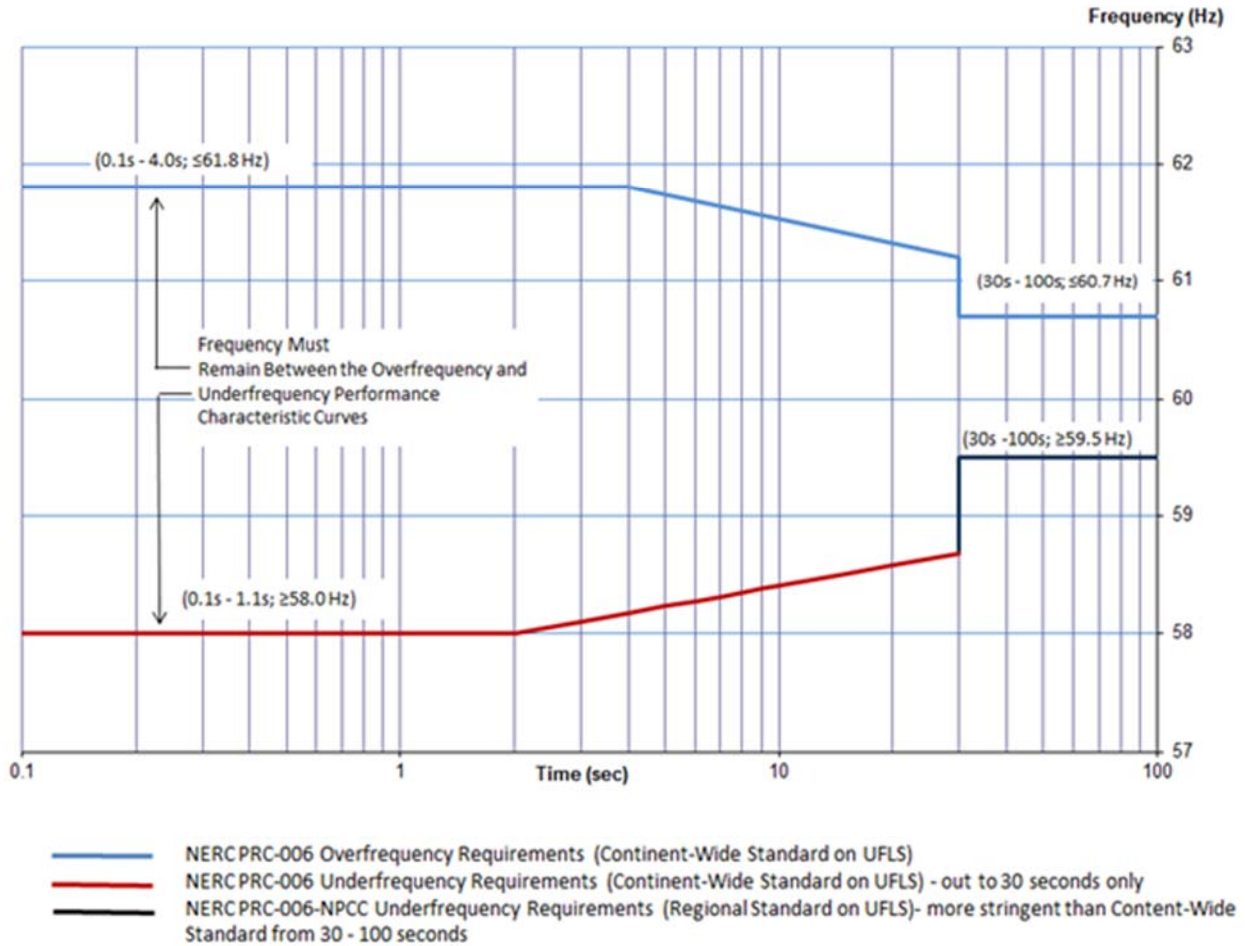
Figure 1 PRC-006-NPCC-2 Underfrequency Load Shedding Program - Eastern Interconnection Design Performance Requirements
