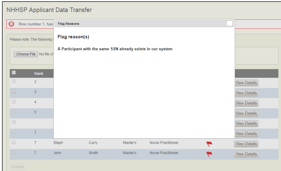
Figure 18: Duplicate SNN in BMISS Flag
