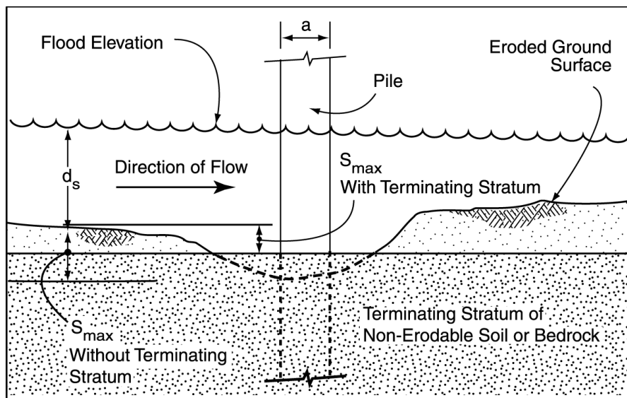
Figure 10 Local Scour
