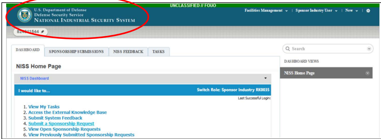
Figure 9. NISS Dashboard
