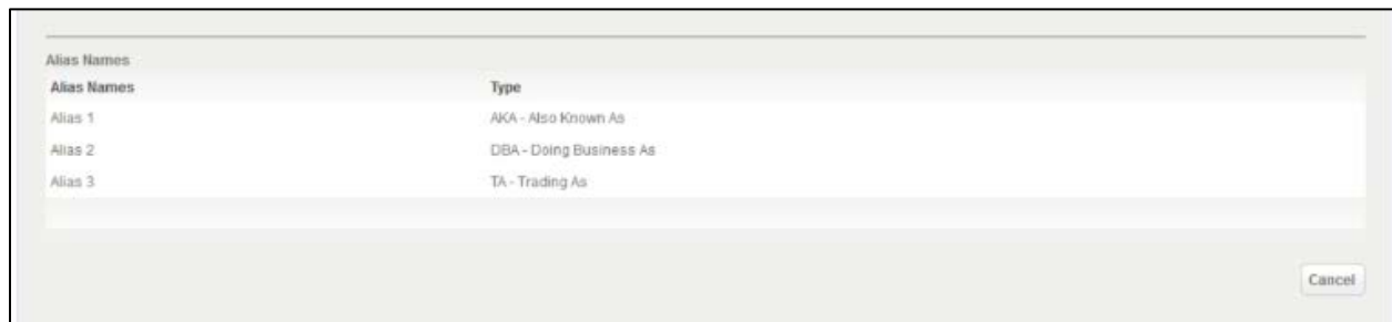
Figure 58. Aliases Page
