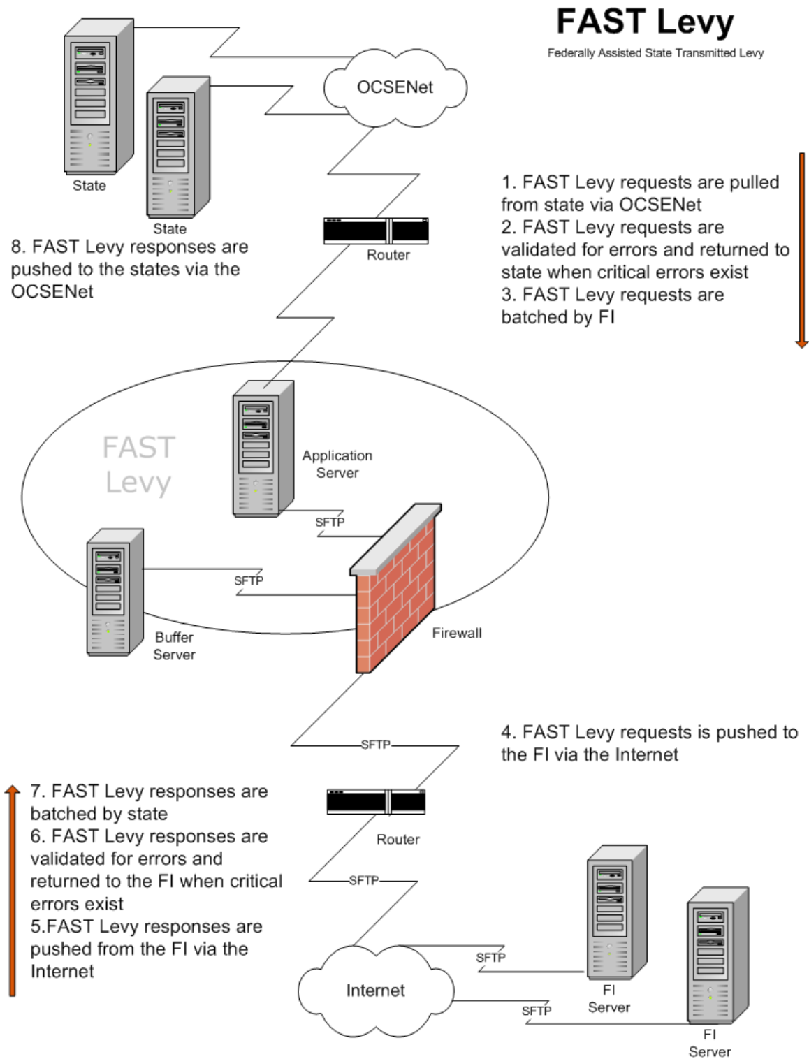
Figure 1-1: Process Diagram
