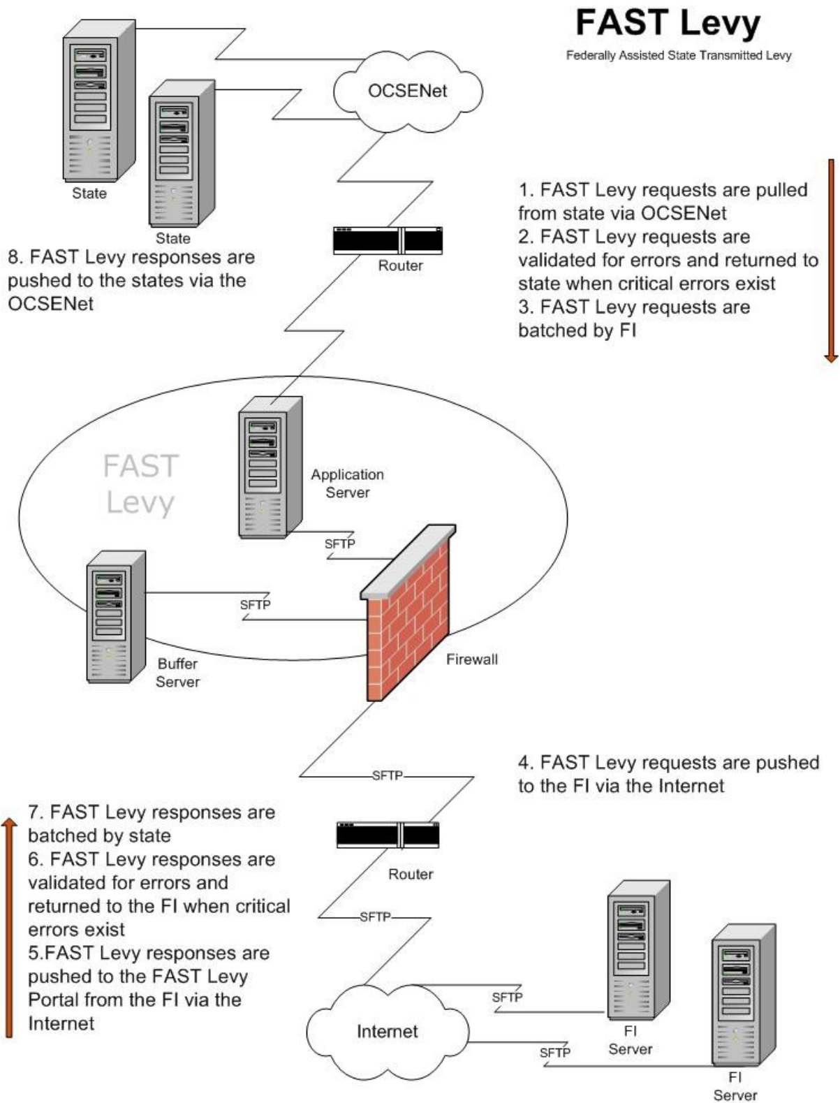
Figure 1-1: Process Diagram
