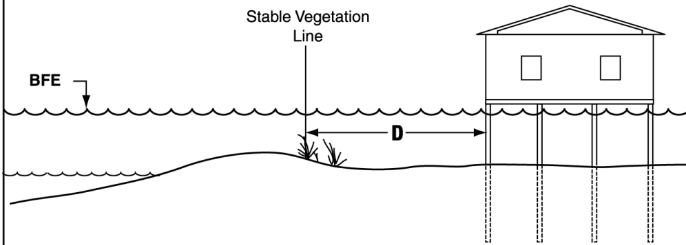
Figure 3 No Dune or Bluff – Use Stable Vegetation Line
