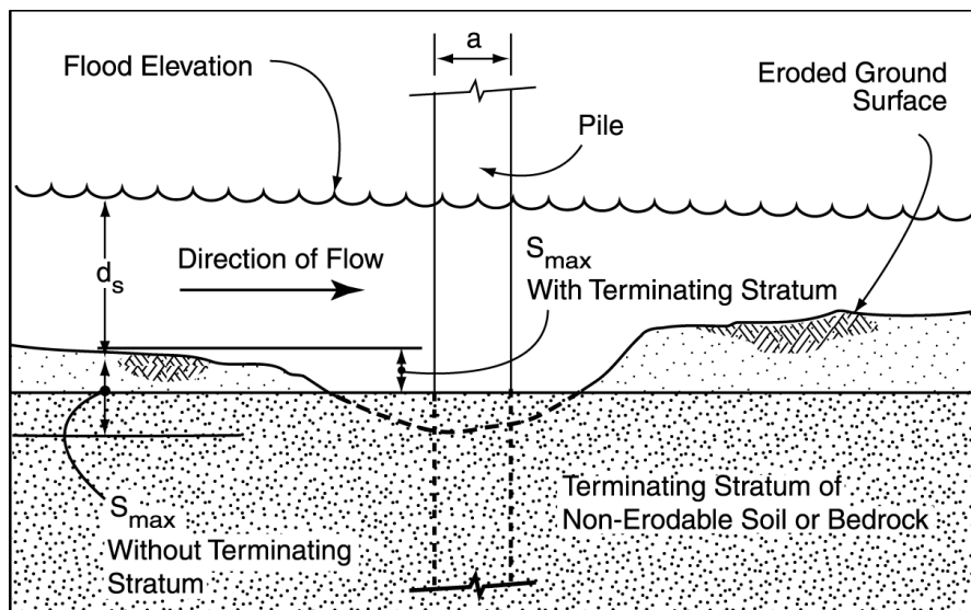
Figure 10 Local Scour
