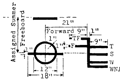
FIGURE 42.13-25(a)—Load line mark and lines to be used with this mark.
