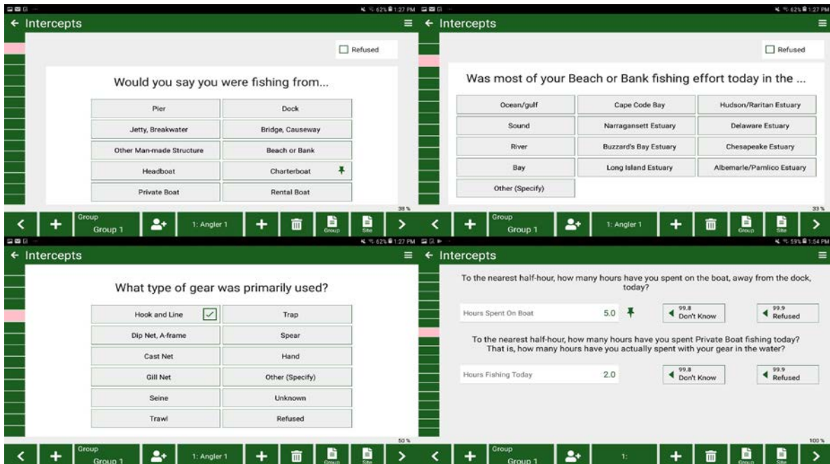
Figure 3. APAIS tablet software screenshots – Angler Interview – Trip Descriptors
