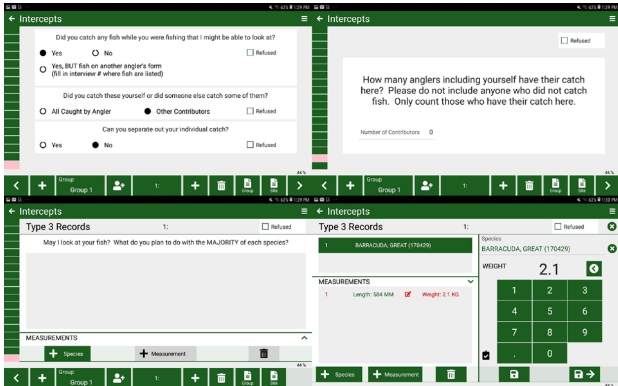
Figure 5. APAIS tablet software screenshots – Angler Interview – Available Catch
