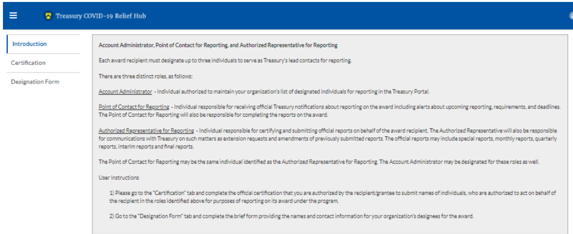
Figure 18 Landing Page
